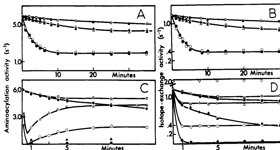
FIGURE 6: Effect of KCl on the tRNA charging and the PP i -ATP isotope-exchange activities of glycyl-tRNA synthetase in the absence and in the presence of DTE. The stock solution of enzyme (1.56 \mu M in the buffer described in Figure 4) was diluted to 93.6 nM in the same buffer containing ( \square , \Delta , \circ , \diamond ) or not ( \blacksquare , \blacktriangle , \bullet ) 20 mM DTE in the absence of KCl ( \square , \blacksquare ) or in the presence of 0.1 M KCl ( \Delta , \blacktriangle ) or 1 M KCl ( \circ , \bullet ). In one experiment ( \diamond ), 1 \mu M tRNA Gly was present in the preincubation mixture. After various preincubation times either at 4 °C (A, B) or at 35 °C (C, D), aliquots were transferred into a complete reaction mixture at 35 °C where the enzyme was further diluted 10 times; the final KCl concentrations were 0.1 M. The initial rates of aminoacylation (A, C) and of isotope exchange (B, D) were determined as described under Experimental Procedures.
