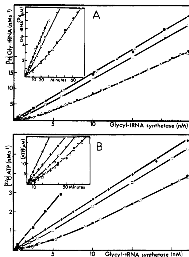
FIGURE 5: Evolution of the glycyl-tRNA synthetase activities as function upon the enzyme concentration in the preincubation mixture and effect of substrates. (A) tRNA charging. (B) PP i -ATP exchange. The stock solution of enzyme ( 1.56 \mu\text{M} in the buffer described in Figure 4) was diluted in the same buffer containing 20 \text{ mM} DTE either in the absence of substrates ( \triangle ) or in the presence of 5 \text{ mM} ATP ( \circ ), 2 \text{ mM} glycine ( \bullet ), 0.1 \text{ mM} \text{Na}_2\text{EDTA} and 5 \text{ mM} ATP plus 2 \text{ mM} glycine ( \square ), 5 \text{ mM} ATP-MgCl 2 plus 2 \text{ mM} glycine ( \diamond ), 1 \mu\text{M} tRNA Gly ( \blacktriangle ), or 1 \mu\text{M} tRNA Phe ( \times ). The glycine was either ^3\text{H} labeled (with the same specific activity as in the aminoacylation mixture) when the tRNA charging was tested or not labeled when the isotope exchange was tested. After 20 \text{ min} of preincubation at 25^\circ\text{C} , the initial rates of both activities were determined at 25^\circ\text{C} , as described under the Experimental Procedures, in reaction mixtures where the enzyme was further diluted twice. In control experiments, the enzyme was directly diluted in the aminoacylation ( \blacksquare ) or in the isotope-exchange mixture containing ( \blacksquare ) or not containing ( \diamond ) 1 \mu\text{M} tRNA Gly . The inset figures represent, respectively, the kinetics of aminoacylation (A) and of isotope exchange (B) after dilution of the synthetase to 2.6 \text{ nM} and preincubation for 20 \text{ min} at 25^\circ\text{C} under the conditions described above.
